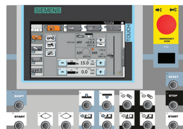
CONTROL PANEL: SIEMENS (X-CNC)
